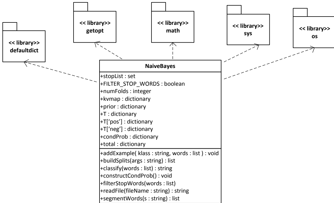
Gambar 7 Diagram kelas Naïve Bayes
